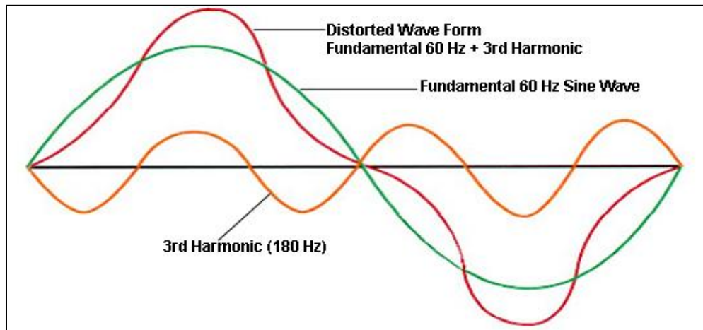
Figure 6: Distorted Waveform Composed of Fundamental and 3 rd Harmonic. THD approximately 30%
