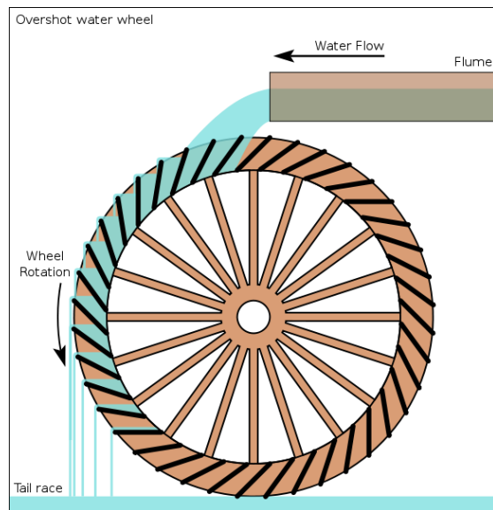
Figure 1: Traditional Water Wheel
