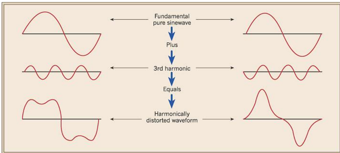
Figure 7: Distorted Wave Forms based on wave forms with different frequency, amplitude and timing.
