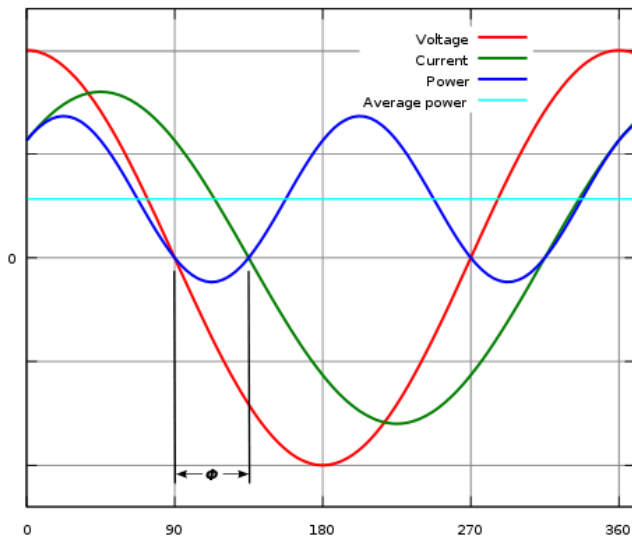
Figure 5: Out-of-Phase Voltage and Current Wave Forms
