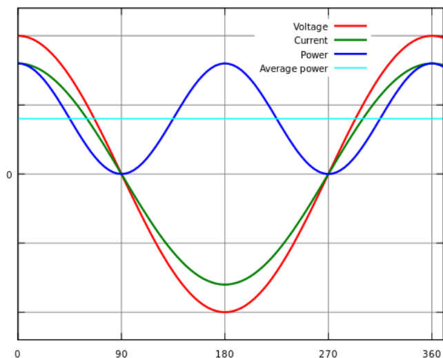
Figure 4: In-Phase Voltage and Current Wave Forms
